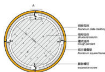
圆形柱子剖面图 (无缝) Circular Column Section (Seamless)
