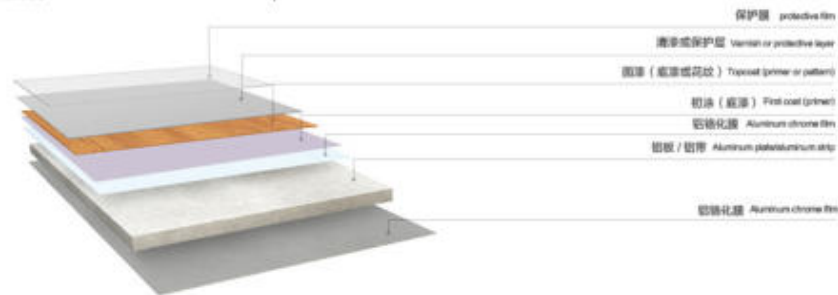
幕墙铝单板产品结构 Curtain wall aluminum veneer product structure
