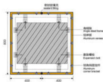
方柱子剖面图 (干挂式) Sectional view of square column (dry hanging type)
